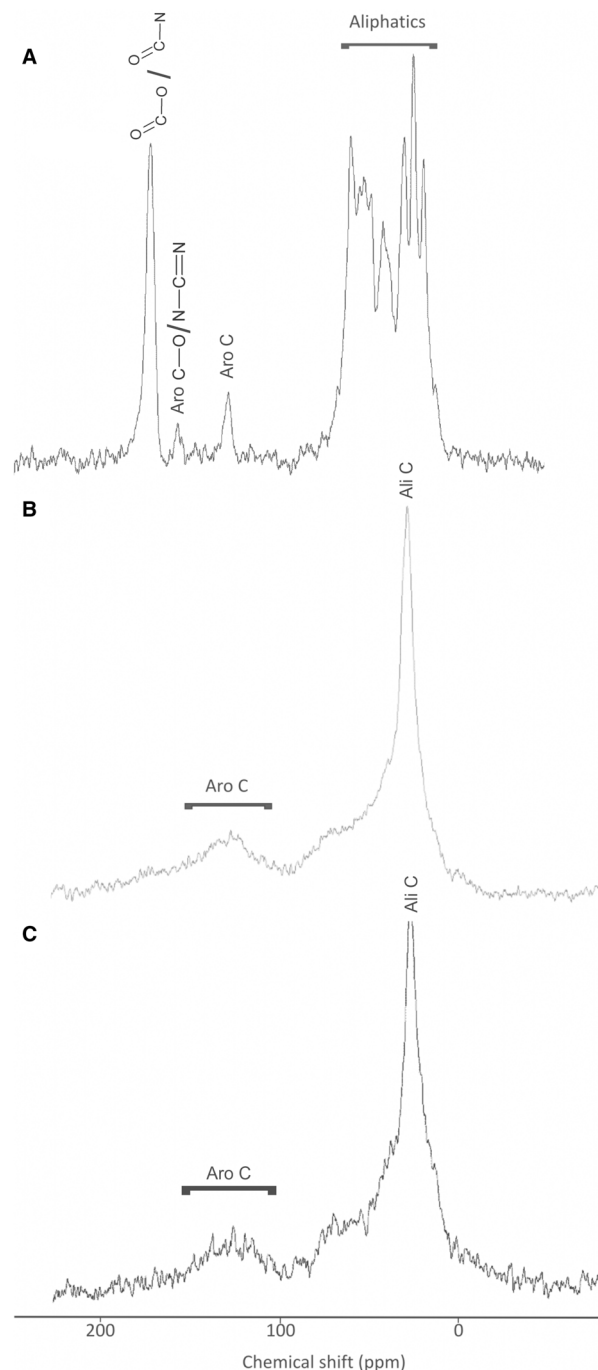
FIG. 6. Cross polarization/magic angle spinning ^{13}\text{C} nuclear magnetic resonance (CP-MAS ^{13}\text{C} NMR) spectra of: A, the modern bird feather; B, the fossil feathers; C, the 'host' sediment. Major chemical functions are indicated on each peak.
